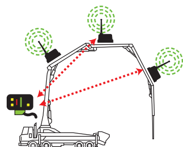
NS/Dualtek with multiple WS sensors
